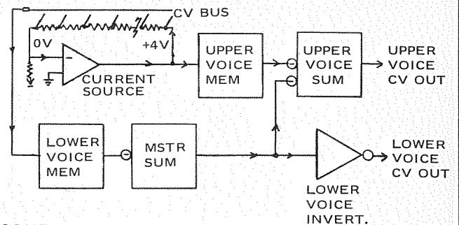
CONTROL VOLTAGE GENERATION
