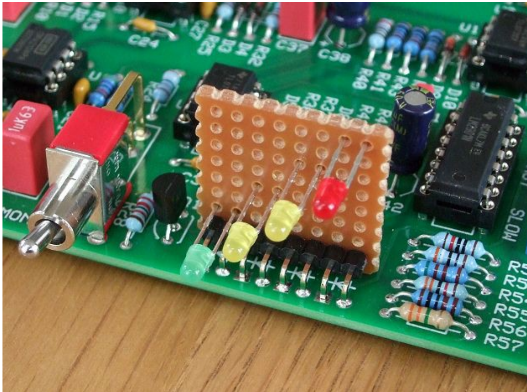
Using stripboard to make the LED connections.
