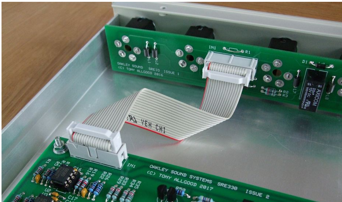
The 16-way ribbon cable used to transfer the balanced audio signals between the SRE330 main board and the SREIO socket board.
