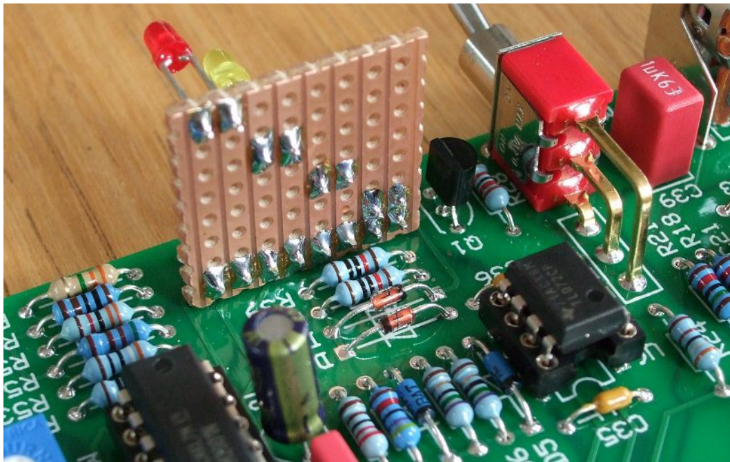
The stripboard's copper strips go vertically. Care must be taken to ensure that the lower edge of the stripboard is properly filed down so no copper tracks can touch the SRE330 main board surface.
