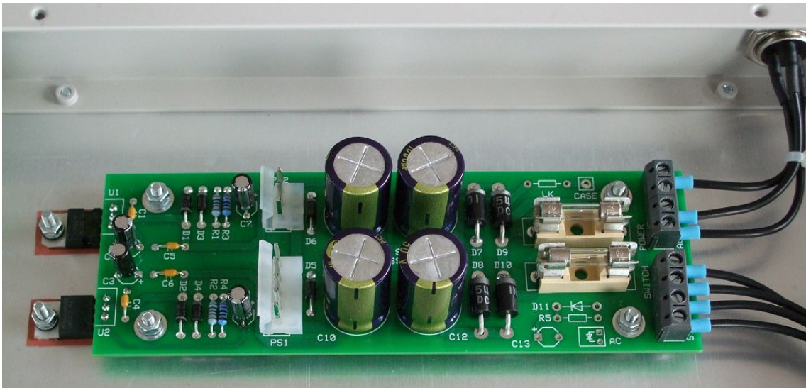
The issue 2 RPSU wired for use with a Yamaha PA-20 external power supply.
