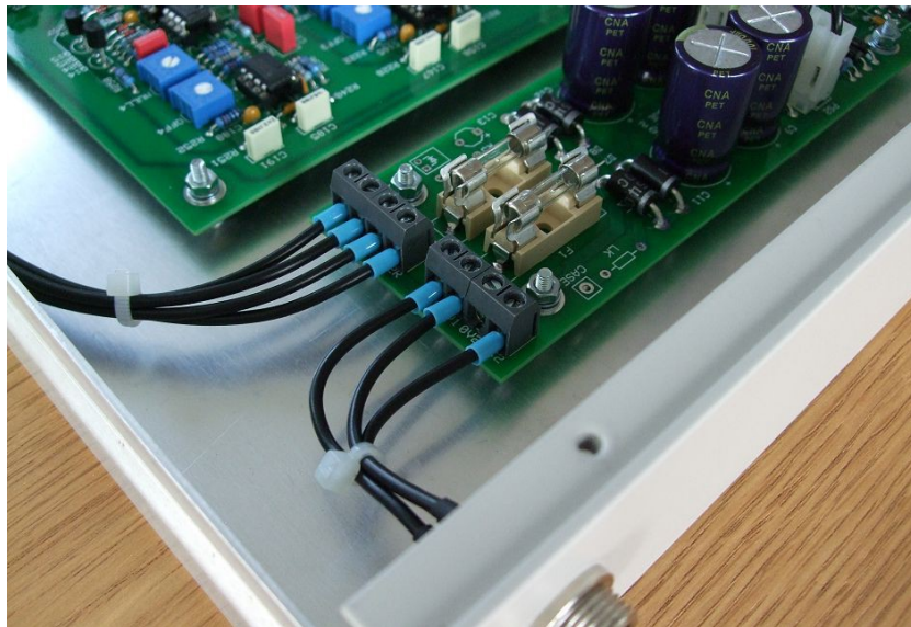
All power wiring uses 24/0.2 insulated wire. I have also boot lace ferrules on the wire ends that go into the terminal blocks for neatness.
